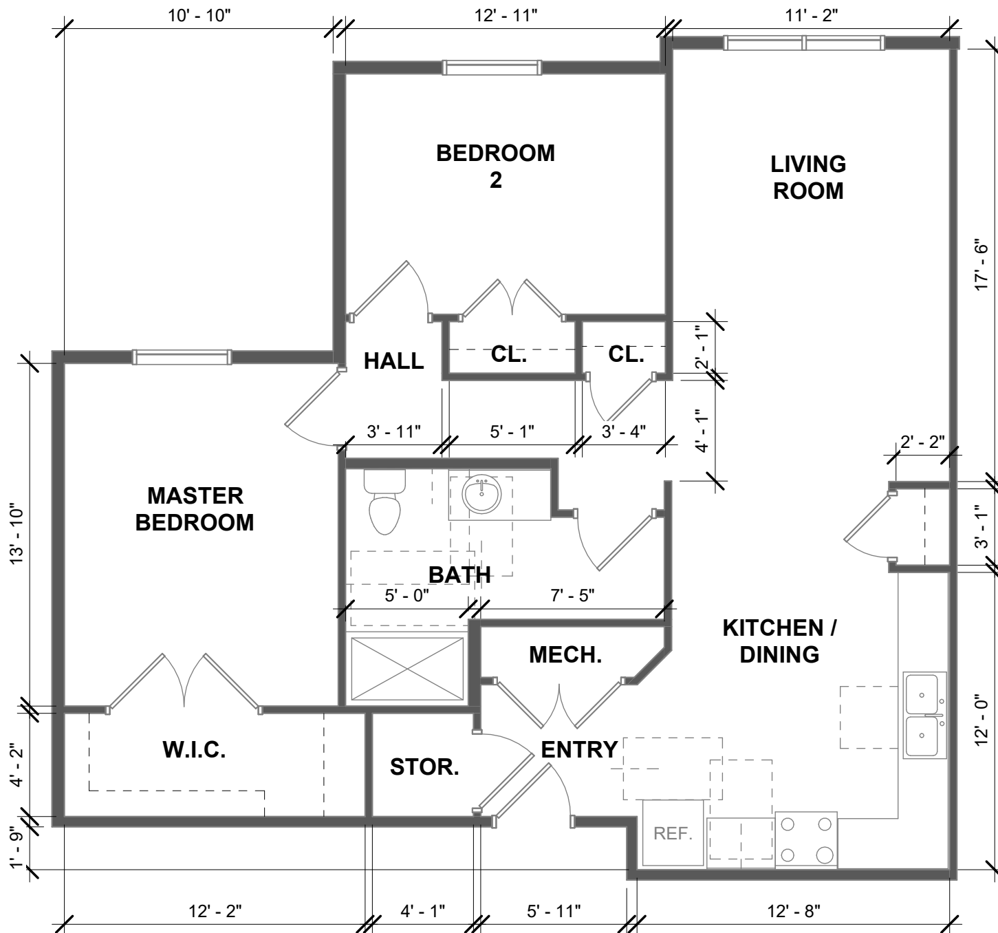
1 TYP. H/C 2 BEDROOM UNIT (TYPE 2) A1.5 3/16" = 1'-0"
