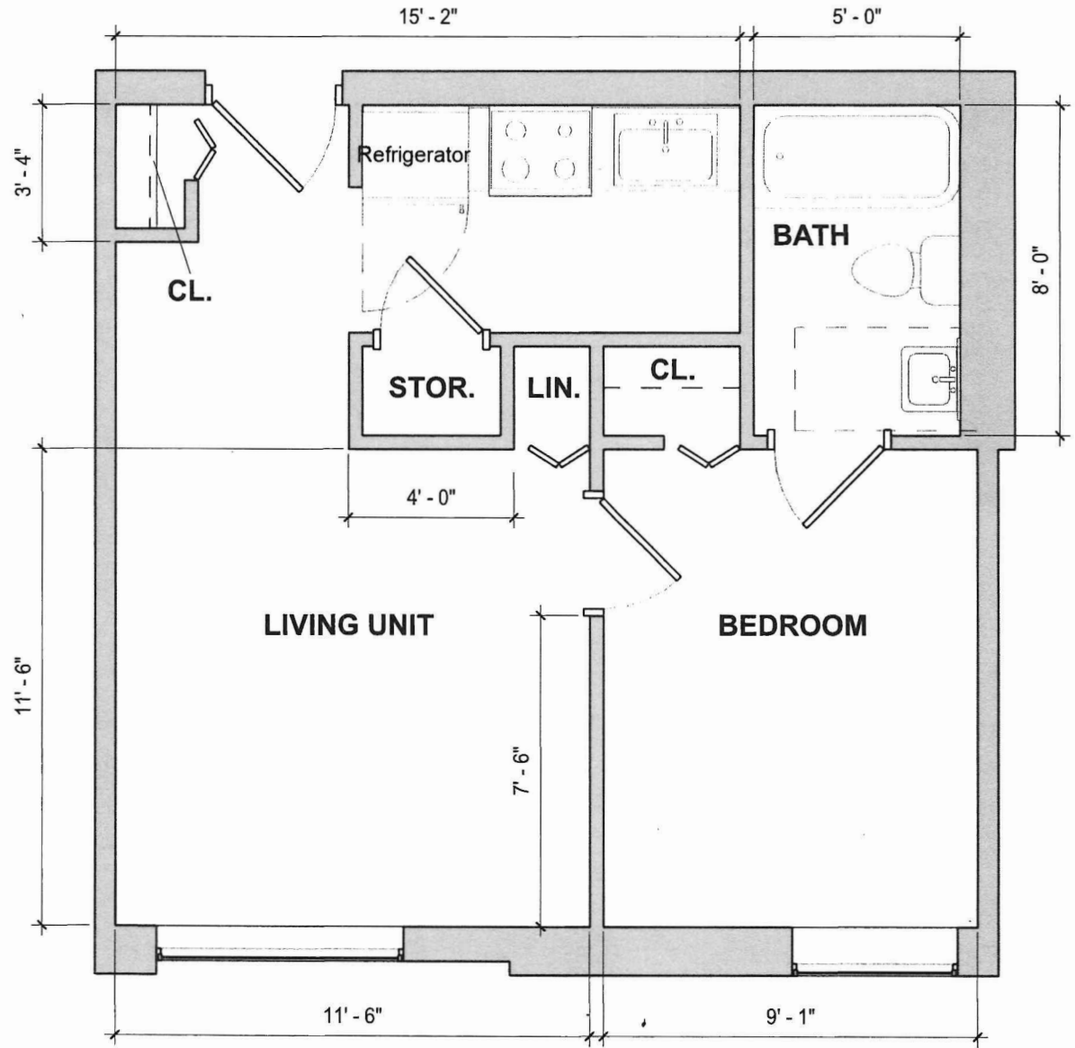
1 TYPICAL EFFICIENCY FLOOR PLAN A1.2 1/4" = 1'-0"
