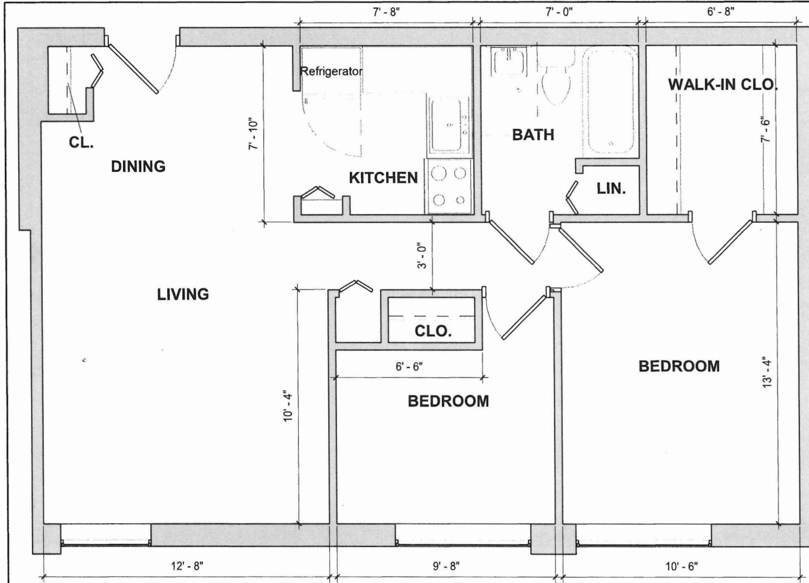
1 TYPICAL 2 BEDROOM FLOOR PLAN (TYPE A) A1.3 1/4" = 1'-0"
